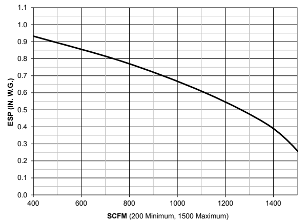
FNP Size 12 with (2) 1/3 HP ECM Motors
