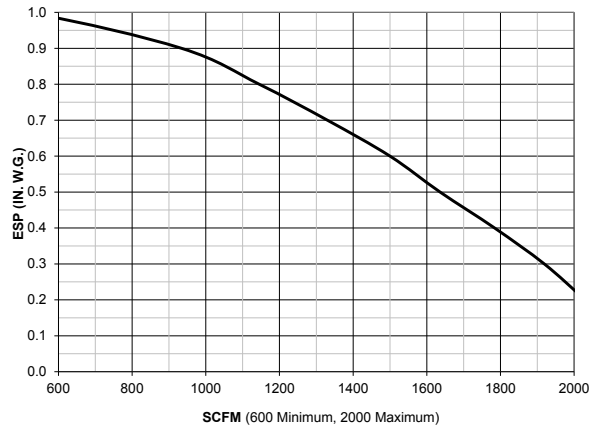
FNP Size 18 & 20 with (2) 1/3 HP ECM Motors
