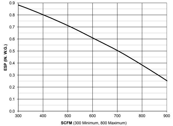
FNP Size 08 with 1/3 HP ECM Motor
