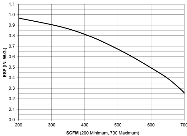
FNP Size 06 with 1/3 HP ECM Motor
