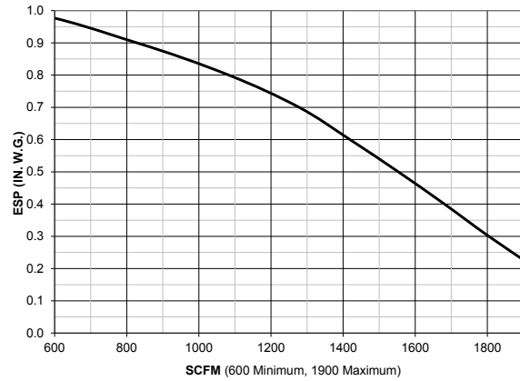
FNP Size 16 with (2) 1/3 HP ECM Motors
