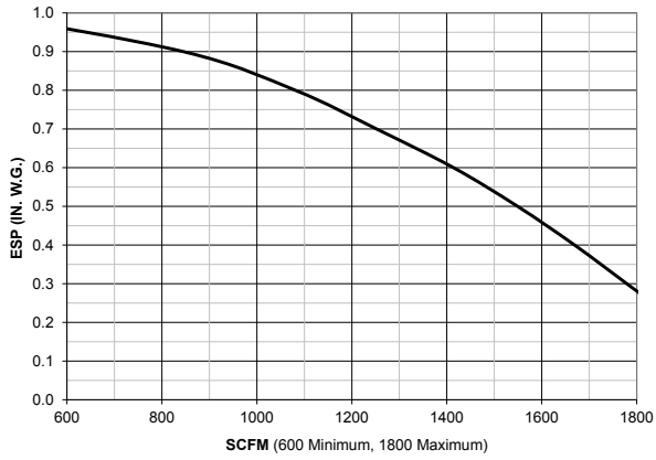
FNP Size 14 with (2) 1/3 HP ECM Motors
