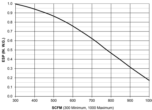
FNP Size 10 with 1/3 HP ECM Motor
